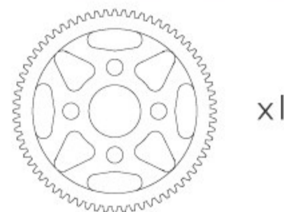
NBA360 Spur Gear 68T (Heavy Duty Steel)
