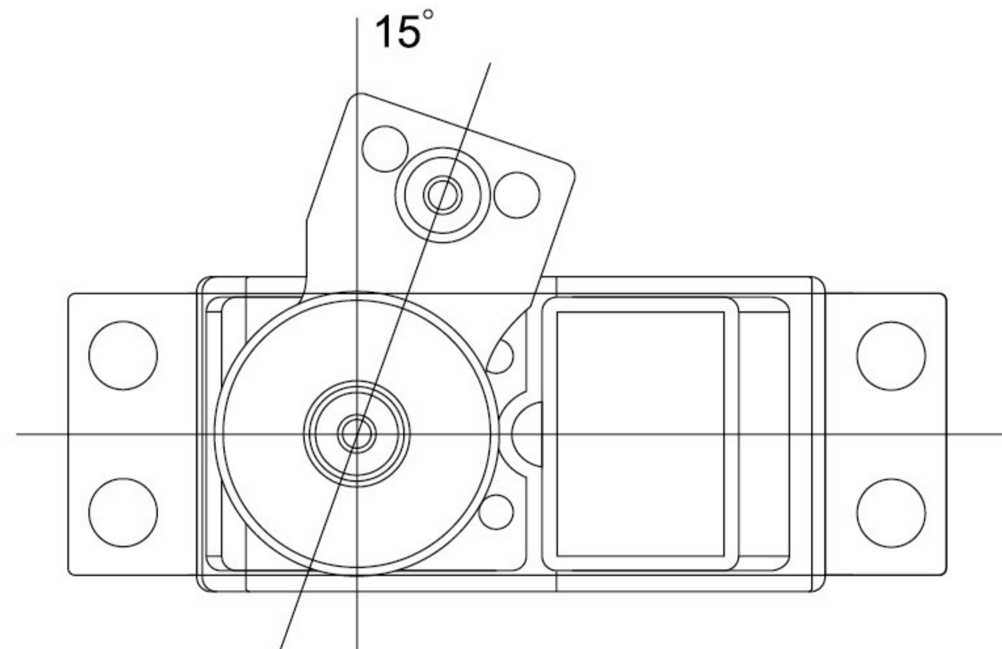
Servo in neutral position and attaching servo saver(15 Degree)
