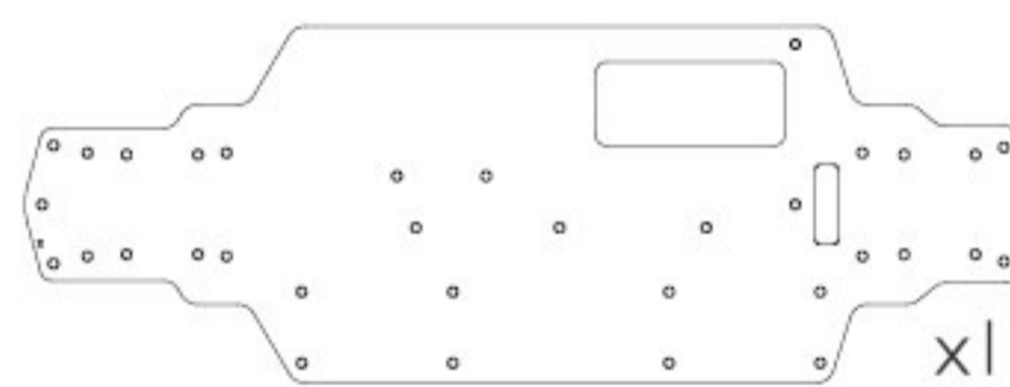
NBA359 M210 Rally chassis AL-7075
